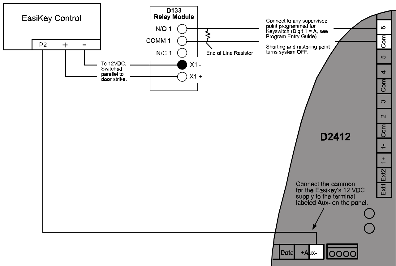
Figure 14: Keyswitch
