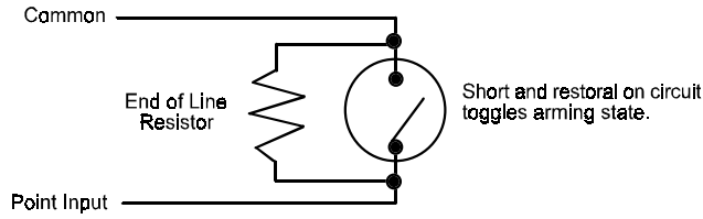
Figure 13: Keyswitch
