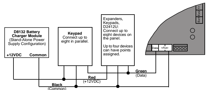
Figure 11: Power for Keypads
