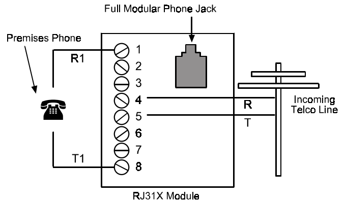
Figure 7: RJ31X Phone Jack
