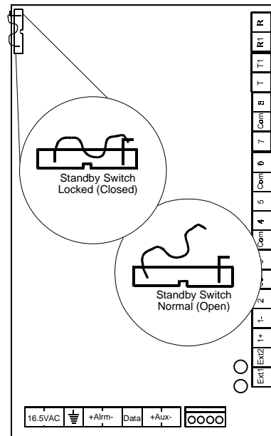
Figure 3: Standby Switch
