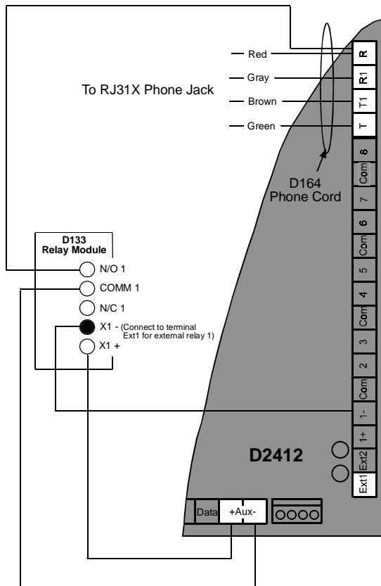
Figure 12: D133 for Ground Start
