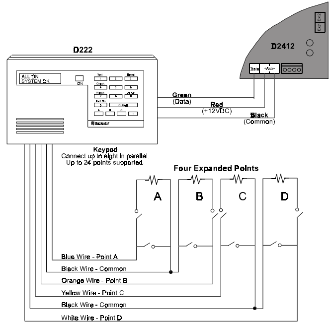
Figure 4: Keypad Wiring
