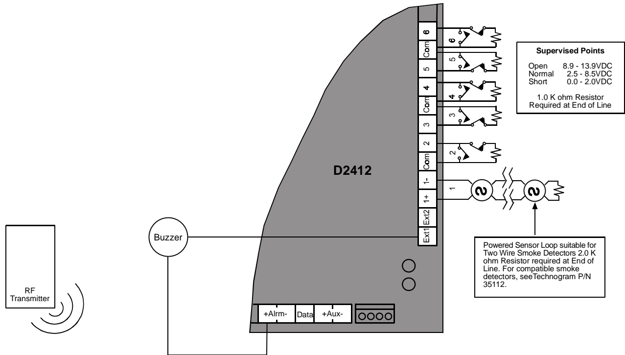
Figure 6: Points
