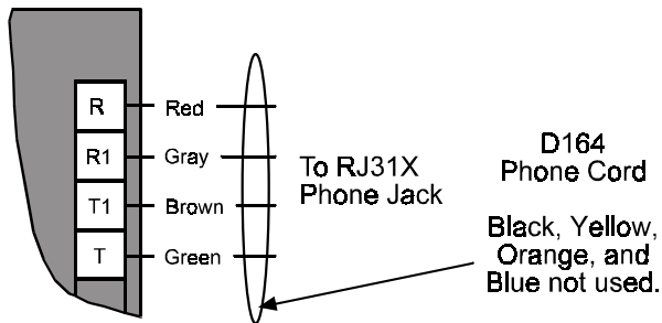
Figure 8: Phone Cord
