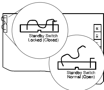
Figure 9: Standby Switch
